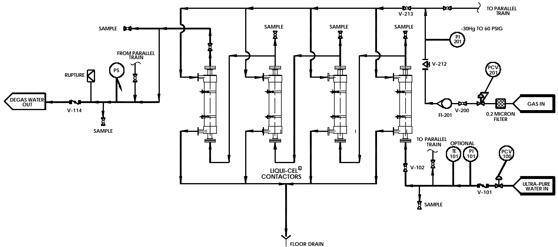
SWEEP MODE VERTICAL USING COMPRESSED GAS SOURCE
